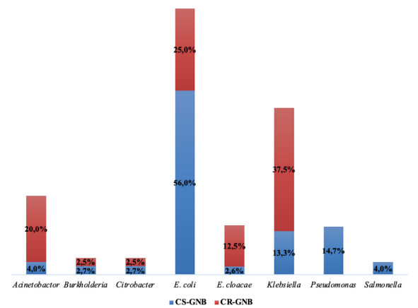
Fig. 1. Distribution of pathogens in patients with CR-GNB and CS-GNB
