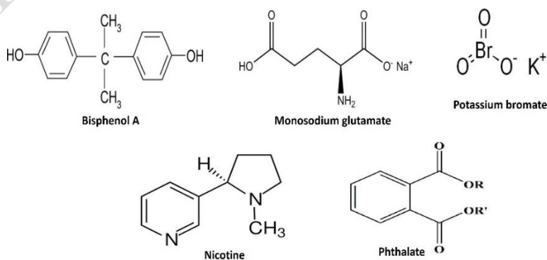
Fig. 2. Structural formula of selected chemicals with testicular toxic effect
