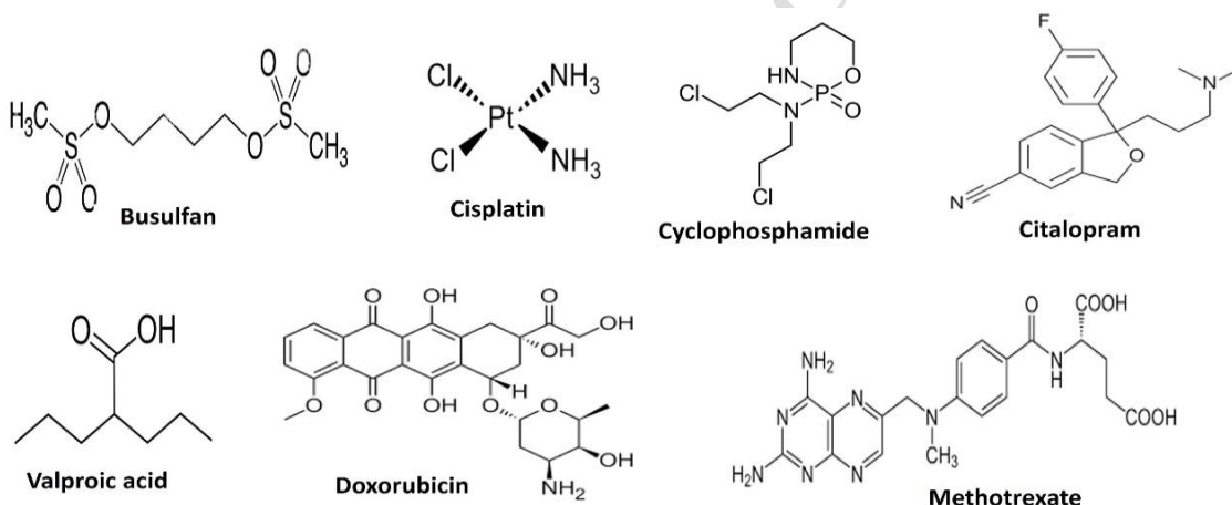
Fig. 1. Structural formula of selected drugs with testicular toxic effect
