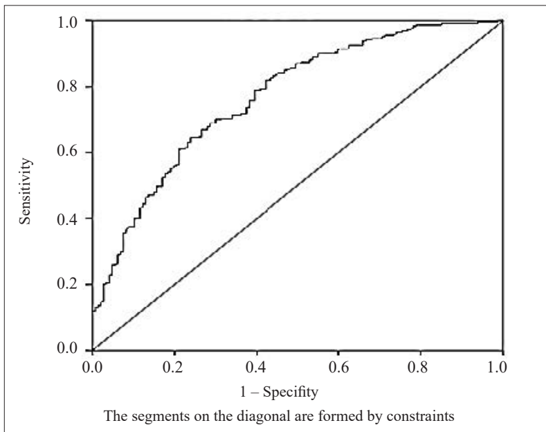
Figure 11. ROC curve
